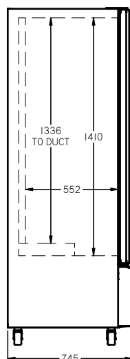
SHELF DETAIL
